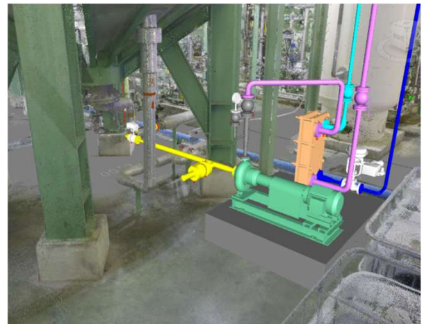
Checking interference by using 3D design
