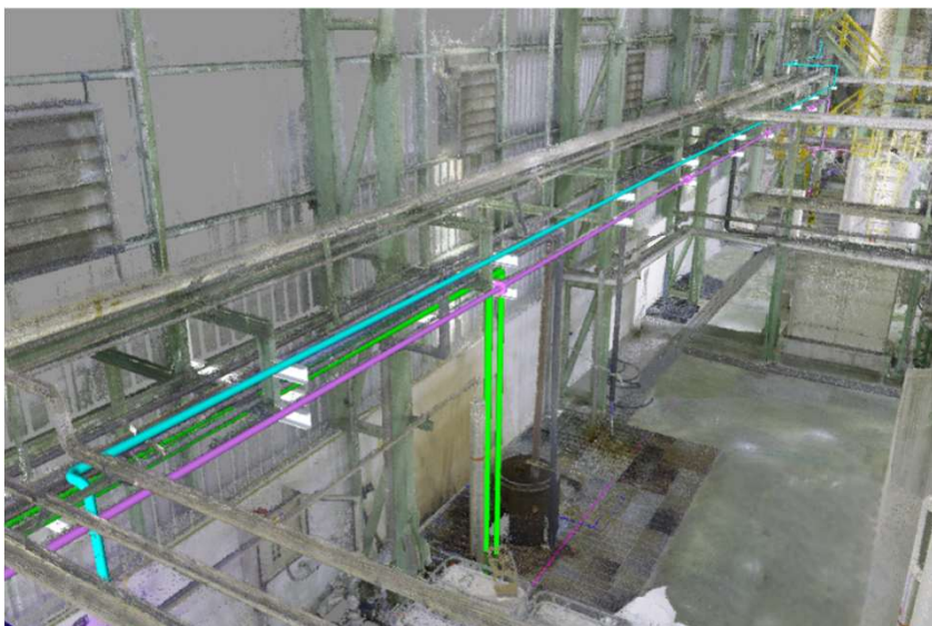
Applied Pipe Rack design on the scanned existing plant data
